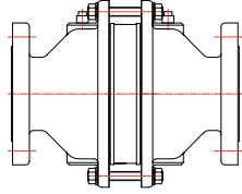
Sockets for Pressure or Thermocouple Tappings
